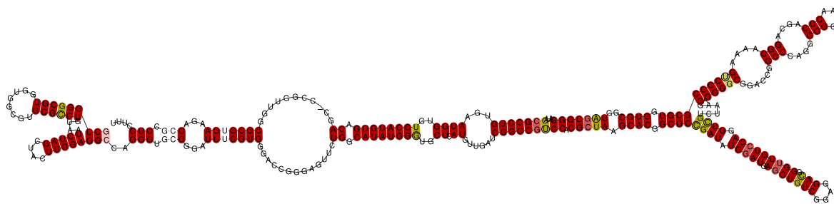
Figure 4: SRP RNA.
