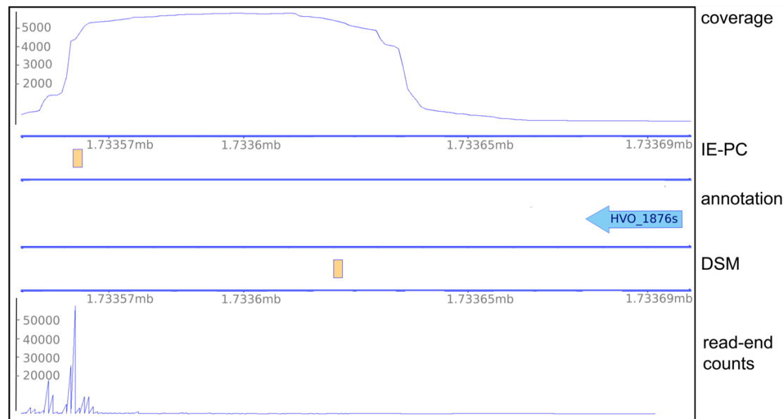
Figure 4. TTS comparison for DSM and IE-PC analyses for the transcript HVO_1876s. The data in the lower panel (DSM) show the DSM results with TTS and corresponding read end counts from the DSM data set. The upper panel (IE-PC) shows the TTS locations determined by IE-PC and the total coverages, corresponding to the -TEX data set. Since sequencing starts at the 3' end, coverage starts at the 3' end and runs continuously for 75 bp due to the read length. The annotation and genome coordinates are shown in the middle (coordinates given in Mb). TTS are shown as orange rectangles.
