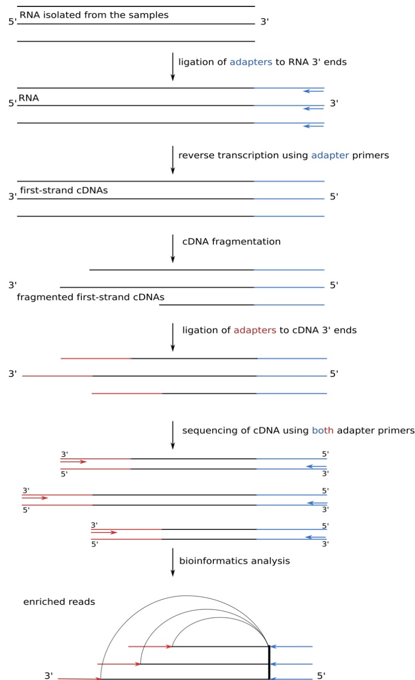
Figure 2. Principle of internal enrichment. After RNA isolation, adapter primers were ligated to the RNA 3' end and the RNA was reverse transcribed. First-strand single-stranded cDNA was fragmented prior to the addition of the adapter primer at the cDNA 3' end (for details, see Materials and Methods and Supplementary Methods). The break points were considered to be random, leading to an enrichment of original RNA 3' ends over 5' fragmentation ends. Sequencing the cDNAs generated from these first-strand cDNA fragments in paired-end mode preserved information about fragment ends, even if they were longer than the read length. After mapping the read-pairs to the reference genome, the hallmark of an original 3' end was its high coverage of read ends, with its associated mate ends originating from a multitude of genomic sites.
