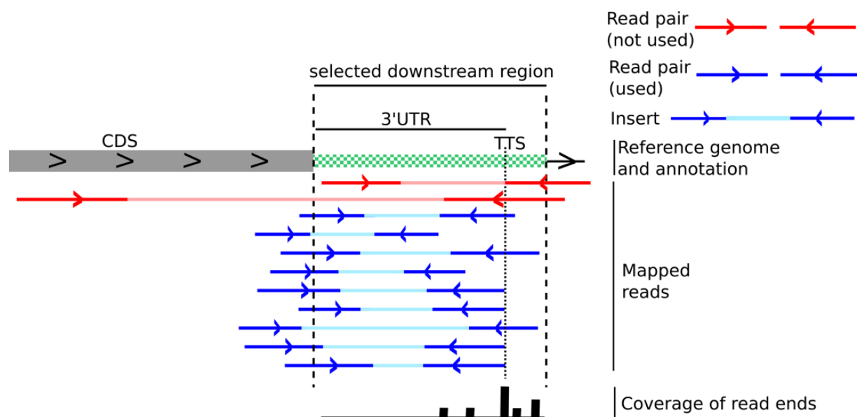
Figure 1. Principle of the Dar-Sorek-Method. As a first step in the DSM method, read pairs with an insert overlapping an annotated region are selected (red and blue lines)(17). Inserts that do not overlap or have a length of more than 500 nucleotides are discarded (red read pairs in the Figure). From the selected read pairs (blue), the average length over all inserts is calculated as described in Dar et al.(17). This value is used to determine the length of the selected downstream region (green white region in the Figure). The coverage of all read ends in this region is retrieved (bottom line), and the position with the highest coverage is identified as the TTS.
