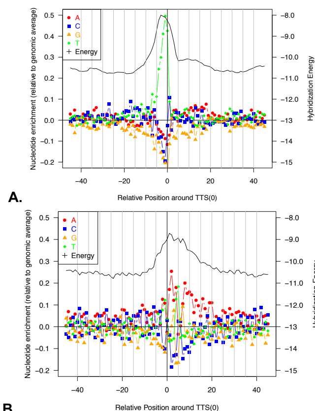
Figure 7. Analysis of up- and downstream regions for TTS identified with IE-PC. A. Intergenic and B. coding regions were investigated. Forty-five nucleotides up- and downstream of the termination site were analysed for (1) nucleotide enrichment at each position (left y-axis) and (2) the hybridisation energy (right y-axis). x-axis: nucleotide position (upstream -, downstream +). The colour scheme for the four nucleotides is shown at the upper left, and the energy data are shown with a black line. Hybridisation energies were calculated based on the binding energies between the DNA template and RNA in the area behind the RNA polymerase. The regular pattern in panel B is due to the statistical characteristics of coding regions in GC-rich organisms(25,26).
