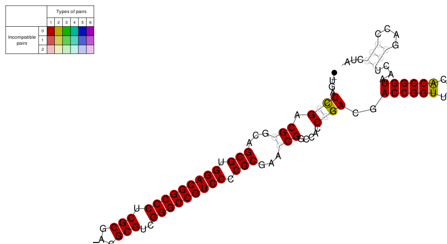
Figure 9. Hairpin structure found upstream of TTS. The secondary structure was plotted with RNAalifold, and its 5' end is denoted by a small dot at the end of the line. The colour coding is at the top left; whereas darker colours show compatible pairs, and the number of types of pairs shows how many types are found at this position thereby indicating sequence conservation. Dark red colours indicate base pairs that are compatible and conserved.
