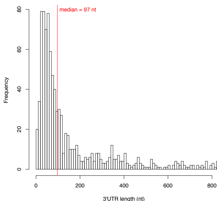
Figure 11. Histogram of 3' UTR lengths. The 3' UTR lengths for all first TTS are shown as calculated from the IE-PC data on the basis of the +TEX reads. The histogram shows the frequency of 3' UTR lengths for the region up to 800 nucleotides in length.
