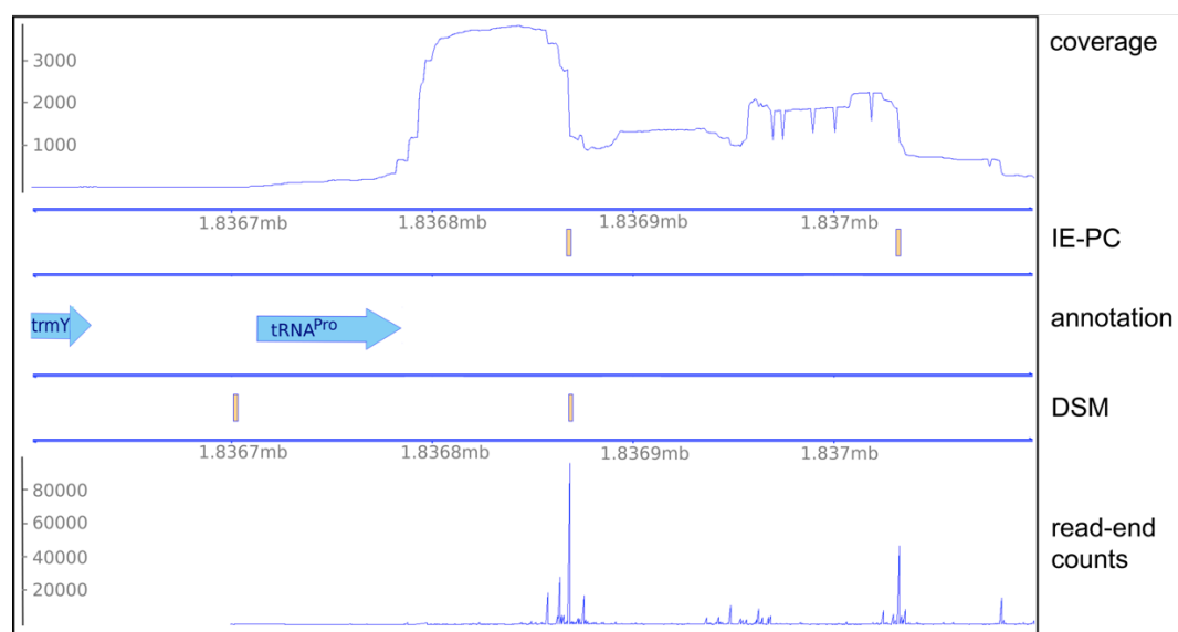
Figure 5. TTS comparison of DSM and IE-PC for the tRNA^{Pro} gene. In the lower panel, termination sites and corresponding read end coverages from the DSM data set are shown, assigning a TTS downstream of the trmY gene and another one downstream of the tRNA^{Pro} gene (shown as orange rectangles). The upper panel shows the TTS location determined by IE-PC and the total coverages, corresponding to the -TEX data set, identifying two TTS downstream of the tRNA^{Pro} gene. Since sequencing starts at the 3' end, coverage starts at the 3' end and runs continuously for 75 bp due to the read length. The secondary TTS of the tRNA^{Pro} gene was not reported by the DSM algorithm as this algorithm systematically reports only a single TTS for each annotated gene.
