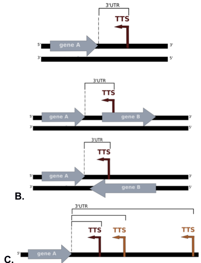
Figure 6. Location of TTS. A. TTS is located in an intergenic region. B. Location of the TTS in an annotated gene that is located on the sense or antisense strand. The length of the UTR was in all cases measured as the distance between the TTS and the 3' end of the upstream annotated gene on the same strand. C. A first (dark brown) and two secondary TTS (light brown) are shown.
