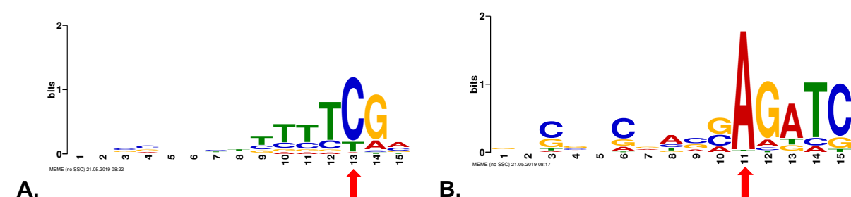
Figure 8. Enriched sequence motifs around the TTS identified with IE-PC. A. Sequence motif close to TTS located in intergenic regions. The TTS is located at position 13 (red arrow). B. Sequence motif close to TTS located in coding regions. The TTS is located at position 11 (red arrow). Motifs were detected using MEME (27).
