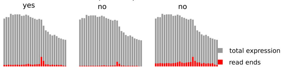
Figure 3. Principle of the applied peak calling procedure. In a sliding window approach, positions where the number of read stops (red) exceeded the mean number of read stops over the whole window by a z-score above the threshold 2 were treated as potential endings (left), while potential peaks of the same height but below a z-score of 2 were discarded (right). In addition, if the number of read stops was below a 10% threshold relative to the total coverage (grey), the peak was discarded (centre).
