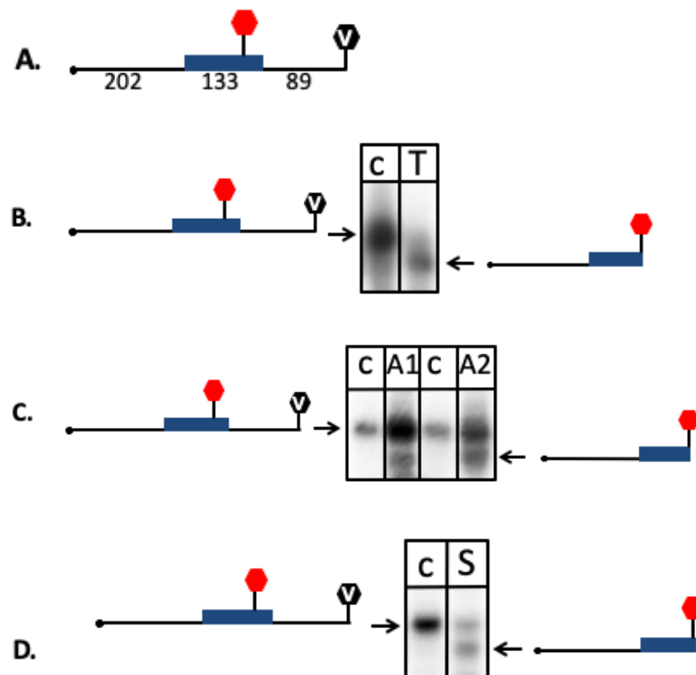
Figure 10. In vivo reporter gene test of termination sites. Termination sites were cloned into a reporter gene (the gene for \beta -galactosidase) construct to confirm their termination activity. RNA was isolated from strains transformed with reporter gene plasmids, separated by size and subsequently transferred to a nylon membrane. Membranes were hybridised with a probe against the \beta -galactosidase mRNA. Active termination sites generated shorter RNA molecules than the control sequences, indicated by an arrow. Experiments were carried out in triplicate. A. The construct used is shown schematically. A full length transcript terminating at the vector termination site is 424 nucleotides long. The insert containing the termination site is 133 nucleotides long (the insert is shown in blue, the location of the termination site in the insert is indicated with a red hexagon), the transcribed plasmid sequences are 202 nucleotides (upstream of the insert) and 89 nucleotides (downstream of the insert) long. The termination site in the plasmid is indicated with a V in the black hexagonal. B. The T 5 C termination sequence was inserted into the reporter gene. Such a T 5 C sequence can be found for example in the intergenic sequence downstream of the fts2 gene. Transcripts terminating at the T 5 C motif are 321 nucleotides long. The T stretch terminated efficiently (indicated with an arrow) with 95% termination at the T stretch and 5% termination at the plasmid encoded terminator (lane T), lane co: control insert without a termination site. C. Two sequences with the downstream motif AGATC (A1 and A2) were inserted into the reporter gene. Both are located in coding regions; A1 is located in the gene HVO_2724, A2 is located in the gene HVO_0455. Termination at these motifs results in 309 nucleotide long RNAs. Both sequences terminated, however considerable read-through is present (termination at A1: 11% and at A2: 27%). Lane A1: AGATC termination site A1, lane A2: AGATC termination site A2. D. A sequence with the potential to fold into a hairpin structure (S12) was inserted into the reporter gene. The structure S12 is located in a coding region (gene HVO_A0420). Termination at this motif results in a 309 nucleotide long RNA. S12 terminated, but considerable read-through was observed (termination at S12: 59%). Lane S: sequence S12.
