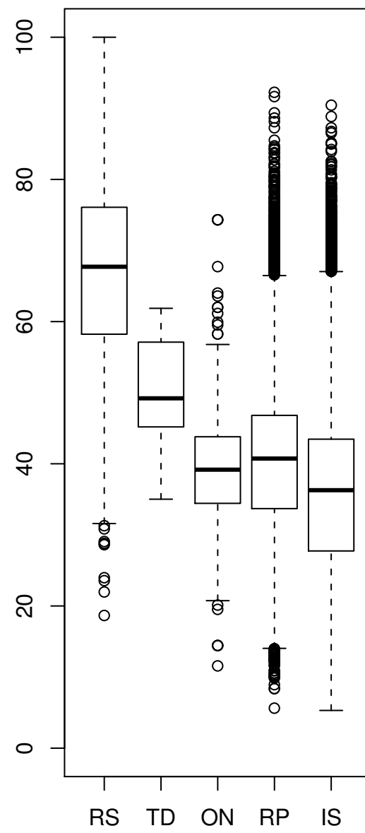
(E) Partial Acceptor (-13 to -3)
