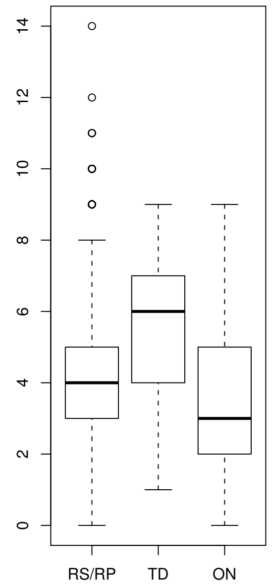
(G) Partial Site Identities
