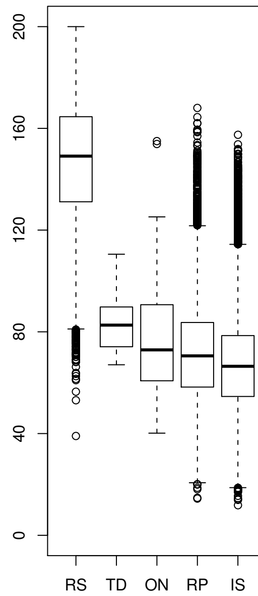
(F) Partial Donor+Acceptor
