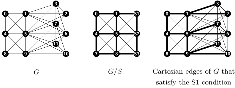
FIGURE 3. This figure shows how we identify (a couple of) Cartesian edges that satisfy the S1-condition . Given a graph G compute its quotientgraph G/S , decompose G/S w.r.t. to its strong prime factors. Since G/S is thin the Cartesian edges in G/S are uniquely determined. Apply now Lemma 2.9 to identify all Cartesian edges in G that satisfy the S1-condition in G/S .
