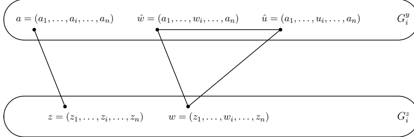
FIGURE 8. N[\hat{w}] \cap V(G_i^y) \subseteq N[w]
