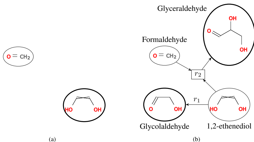
Figure 5 Application of a parallel strategy Q = \mathbf{parallel}[\{r_1, r_2\}] to a graph state F , with r_1 being the transformation rule for the enol to keto conversion and r_2 being the transformation rule for aldol addition (see Appendix A). (a) The reaction network with the graph state F consisting of U(F) = \{\text{formaldehyde, 1,2-ethenediol}\} and S(F) = \{1,2-ethenediol\} . (b) The reaction network after evaluation of Q(F) , with two new molecules; glycolaldehyde and glyceraldehyde. The resulting graph state F' has U(F') = \{\text{formaldehyde, 1,2-ethenediol, glycolaldehyde, glyceraldehyde}\} and S(F') = \{\text{glycolaldehyde, glyceraldehyde}\} . In both networks the subset of the graph state is highlighted (see online version for colours)
